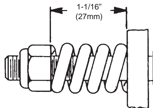
Figure 4-9 Clutch Spring Length
